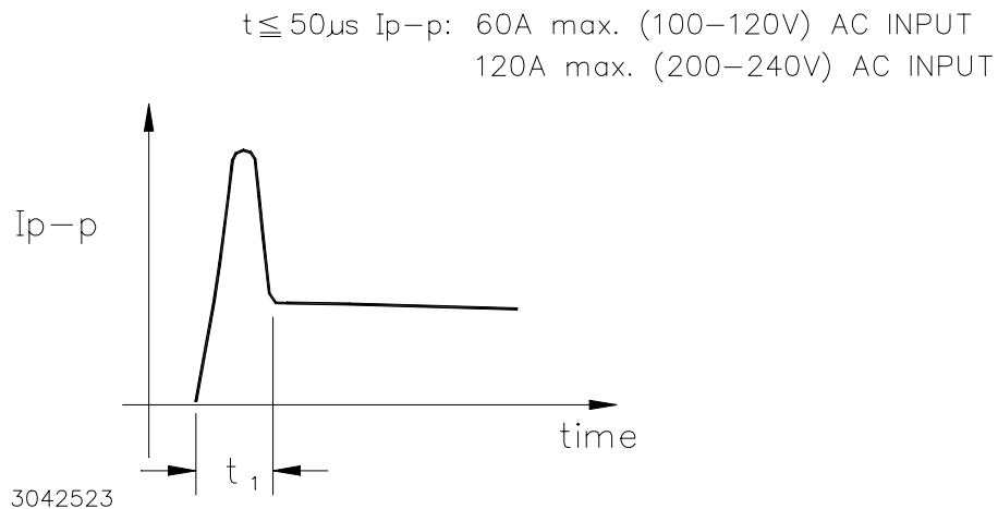
FIGURE 1 RCW 1500W POWER SUPPLY PEAK TO PEAK INPUT SURGE CURRENT FOR T<50US
