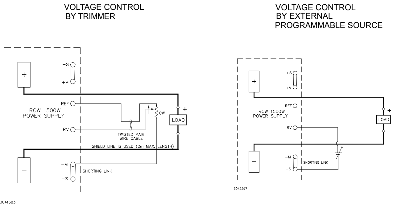
FIGURE 7 CONNECTIONS FOR REMOTE VOLTAGE CONTROL OF THE RCW 1500W POWER SUPPLY
